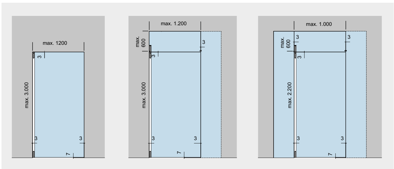
Basic fitting and over panel fitting wall connector for door with over panel and side panel on pivot point side. Optionally with side panel on closing side.
